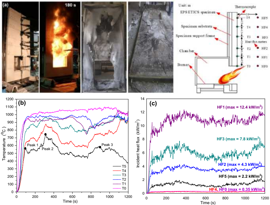
Figure 7. EPS ETICS (thickness = 200 mm) fire test with chamber fire HRR of 1100 kW, (a) samples before and after the test, (b) facade surface temperature, and (c) heat flux in front of facade fire.
