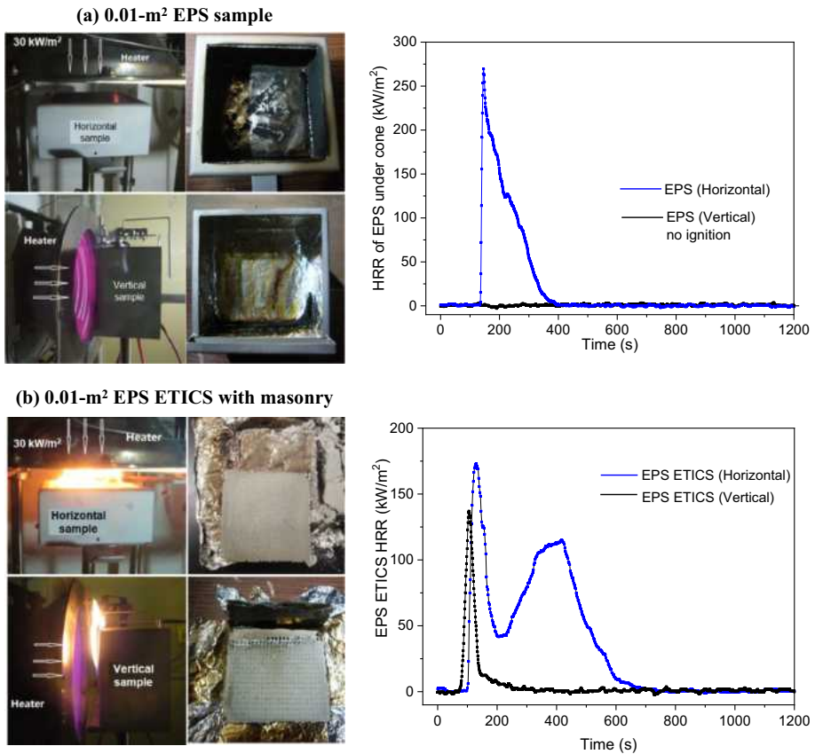
Figure 3. Phenomena and HRR of 0.01-m 2 cone tests under the 30-kW/m 2 irradiation, (a) EPS sample, where no ignition occurs on the vertical sample, and (b) EPS ETICS sample with the masonry cover, where ignition occurs on both horizontal and vertical samples.
