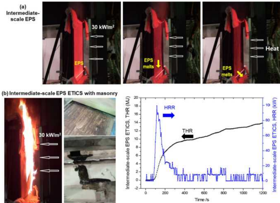
Figure 4. The 1\text{-m}^2 intermediate-scale tests under 30\text{ kW/m}^2 irradiation (a) EPS sample, where no ignition occurs, and all molten fuel flows away (Video S1), (b) EPS ETICS sample with the masonry cover, where ignition occurs, and part of molten EPS flows away (Video S2), and the evolution of fire THR and HRR.
