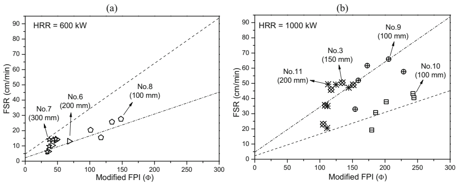
Figure 6. The influence of HRR on FSR versus, (a) 600 kW, and (b) 1000 kW.
