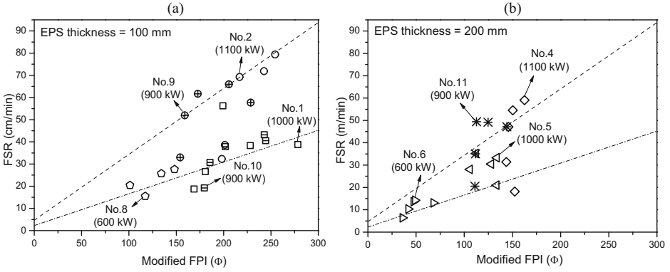
Figure 7. The influence of EPS thickness on FSR versus (a) 100 mm (b) 200 mm.
