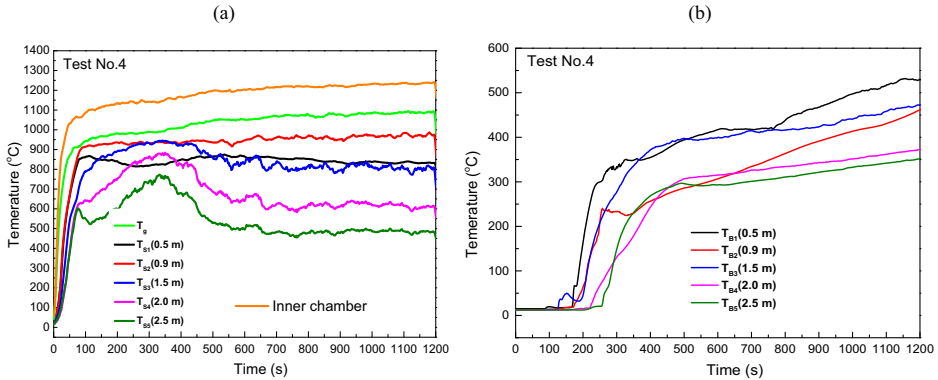
Figure 3. The surface and back temperature histories of No.4 varying with test time, (a) surface temperature ( T_S ), and (b) back temperature ( T_B ).
