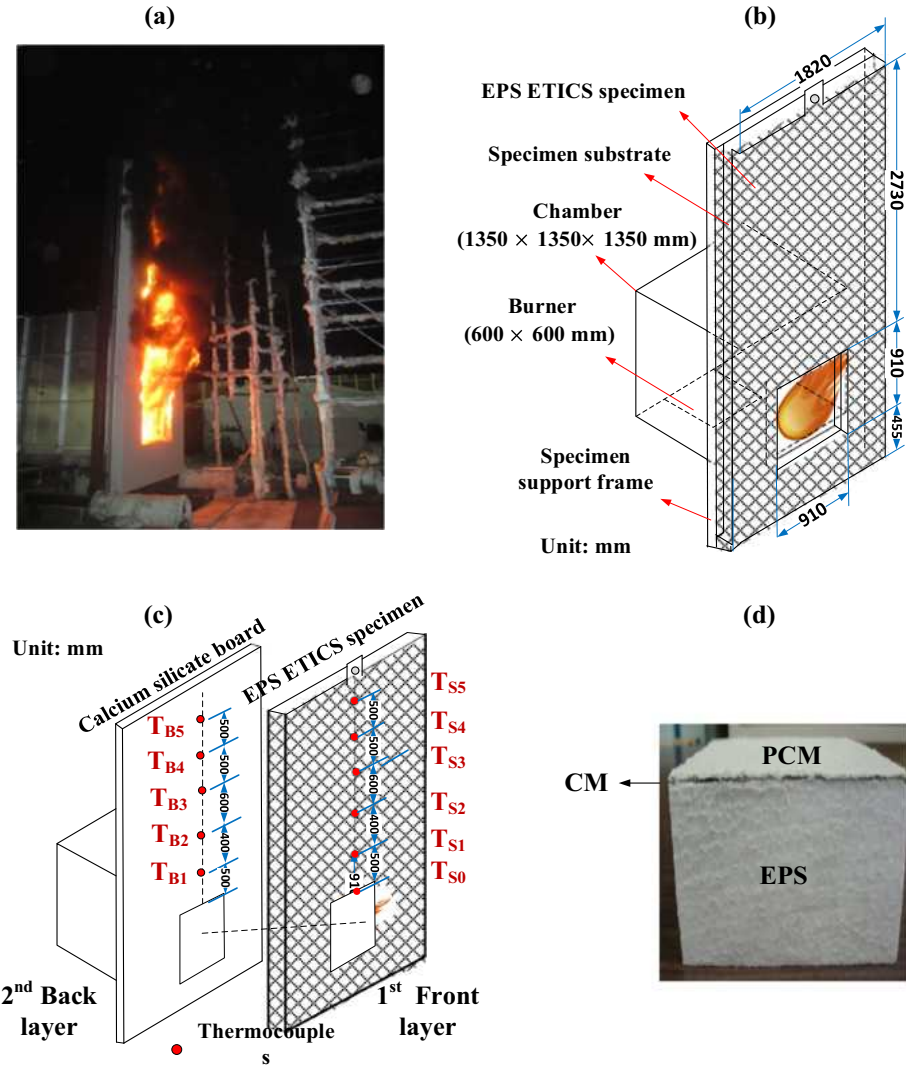
Figure 1. The description of the experiment (a) The layout of test configurations (b) a sketch model of experiment layout (c) thermocouple configuration (d) the details of EPS ETICS configuration.
