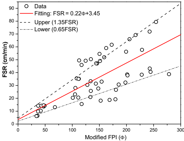
Figure 5. The relationship between FSR of each position and modified FPI ( ).
