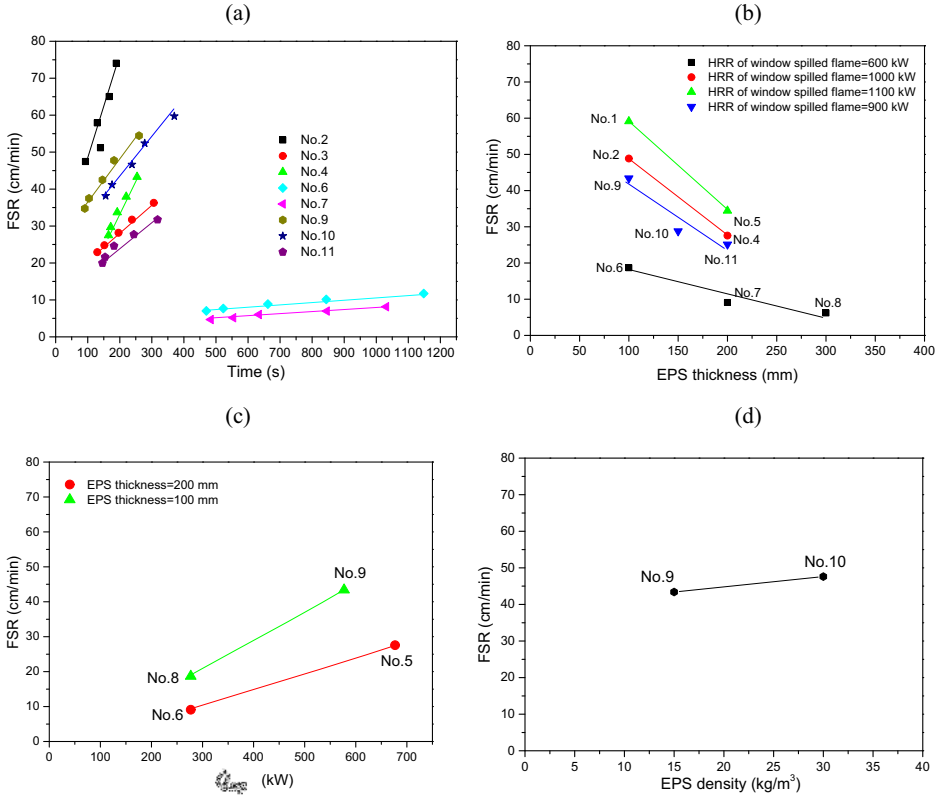
Figure 4. The description of FSR varying test time, EPS thickness, HRR and EPS density, (a) FSR versus test time (b) –FSR versus L_{EPS} (c) –FSR versus \dot{Q}_{sp} (d) –FSR versus \rho_{EPS} .
