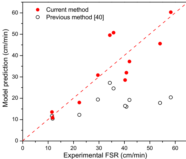
Figure 8. The deviation between experimental and calculated FSR by using two methods.
