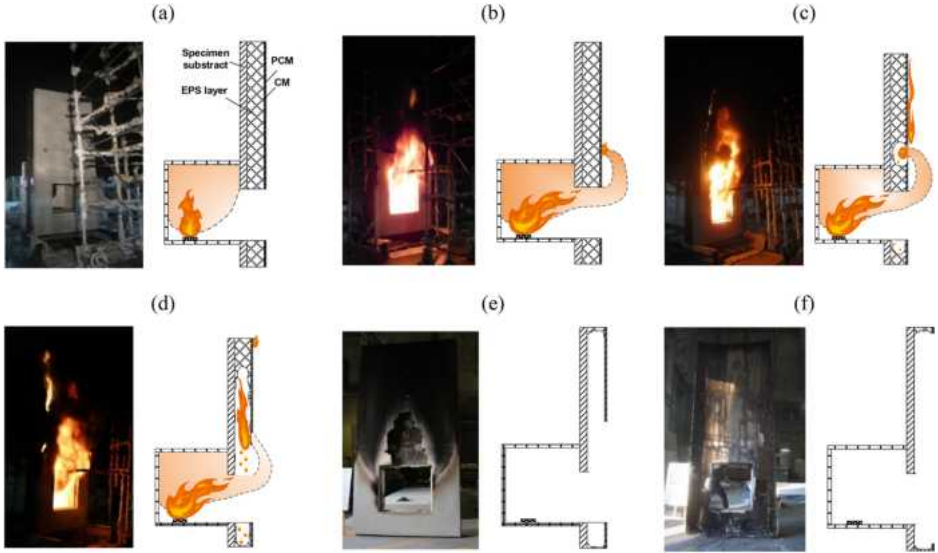
Figure 2. The description of façade fire tests, (a) Early stage at t = 1 s, (b) flame spilled out at t = 24 s, (c) ignition of EPS and the formation of hole in CM layer at t = 95 s, (d) upward flame propagation at t = 326 s, (e) EPS burnout outlook, and (f) removal of façade.
